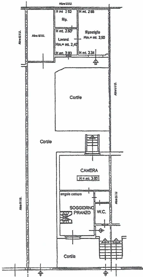
Piano TERRENO
